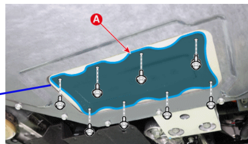
A : BMS ECU service cover
